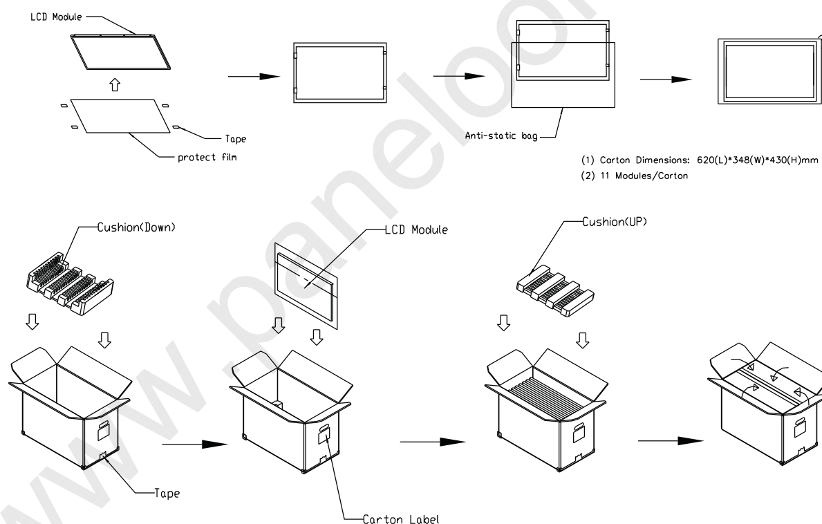
Figure 10-1 packing method
