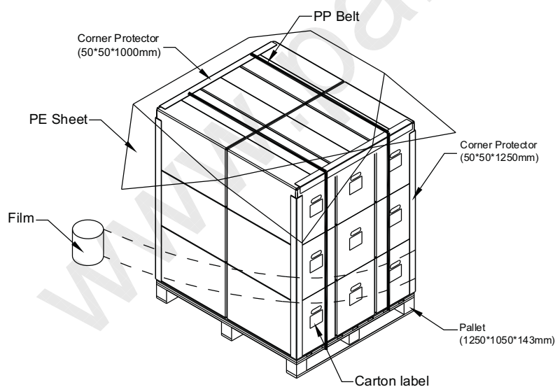
Figure 10-2 packing method
