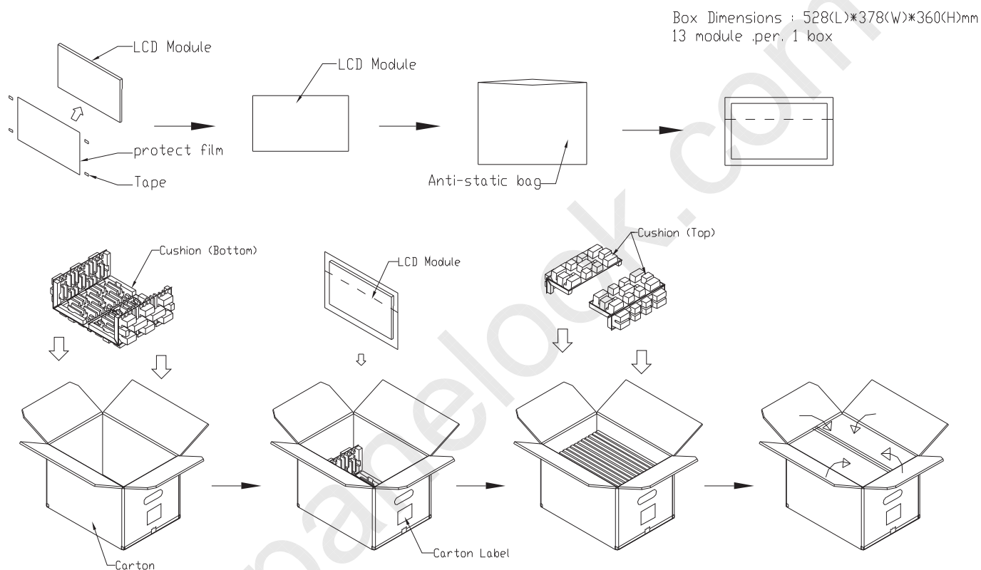
Figure 10-1 packing method
