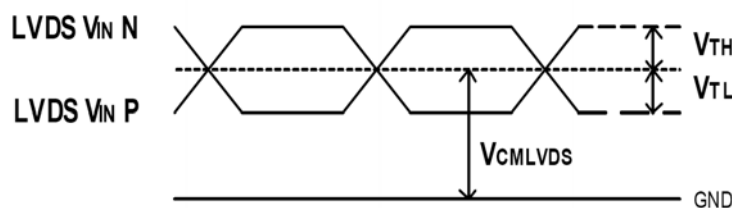
Figure 4.1.1 LVDS DC timing diagram
