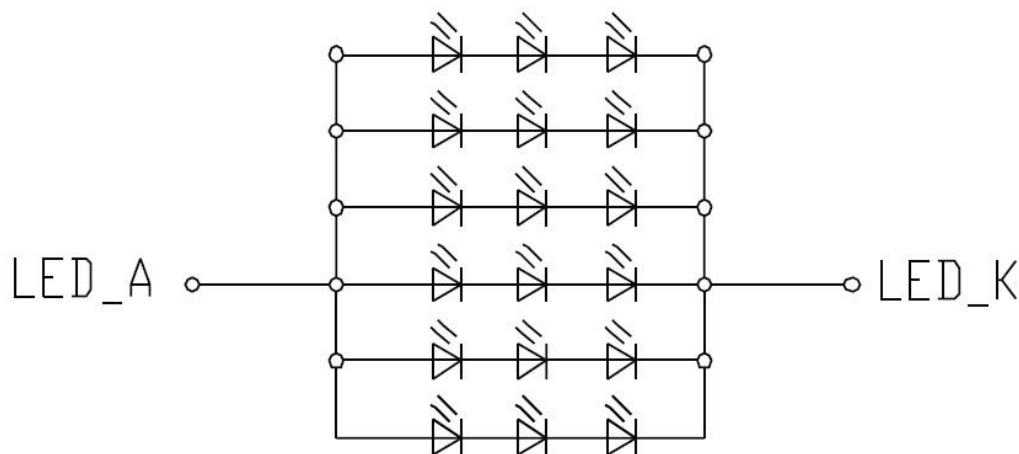
LED circuit
