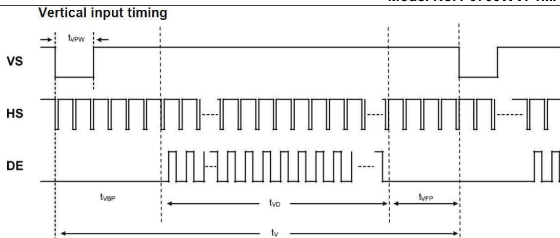
Figure 5.2.2 Vertical input timing
