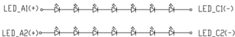
Backlight Circuit Diagram 2*7=14LEDS; I_F=110mA/LED
