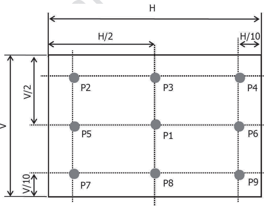
Figure 2. White Luminance and Uniformity Measurement Locations (9 points)
