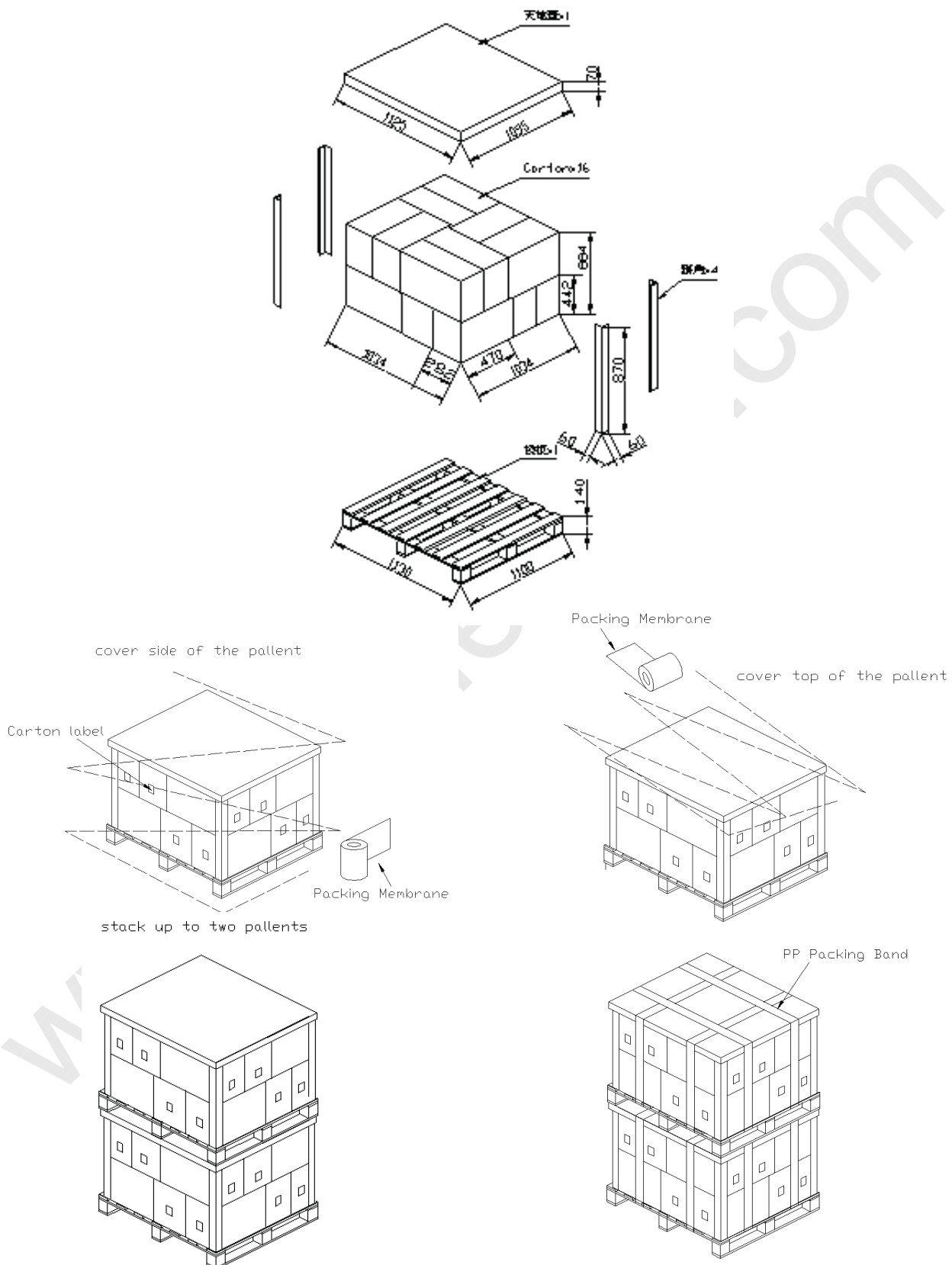
Figure. 7-2 Packing method
