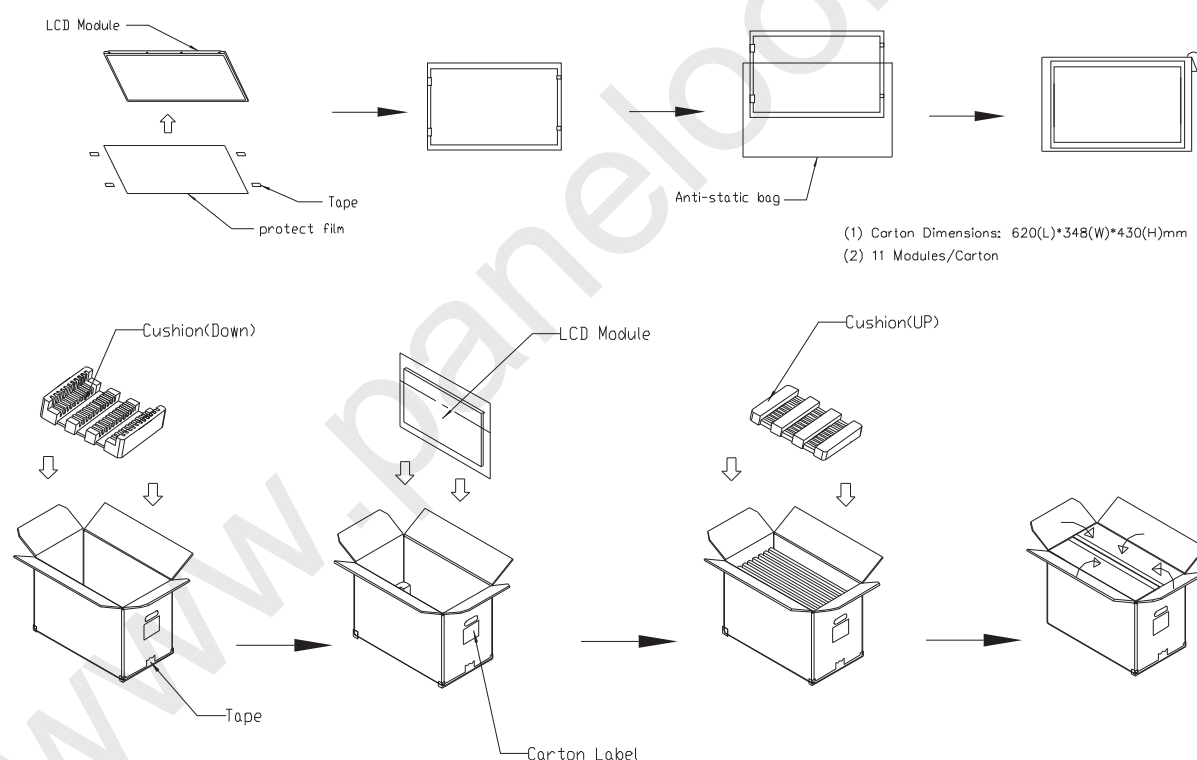
Figure. 7-1 Packing method
