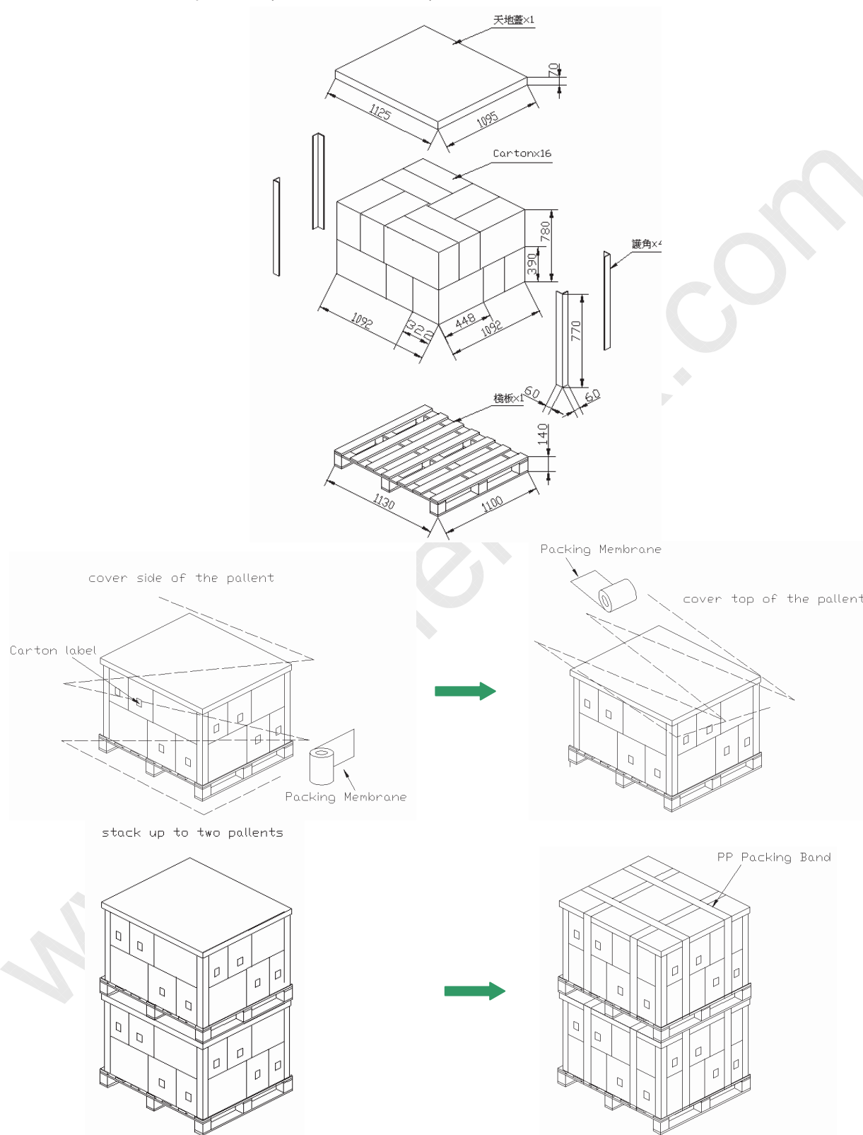
Figure. 7-2 Packing method
