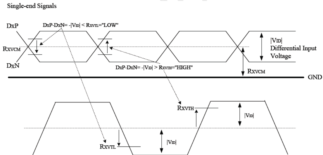
Figure 8 Voltage Definitions
