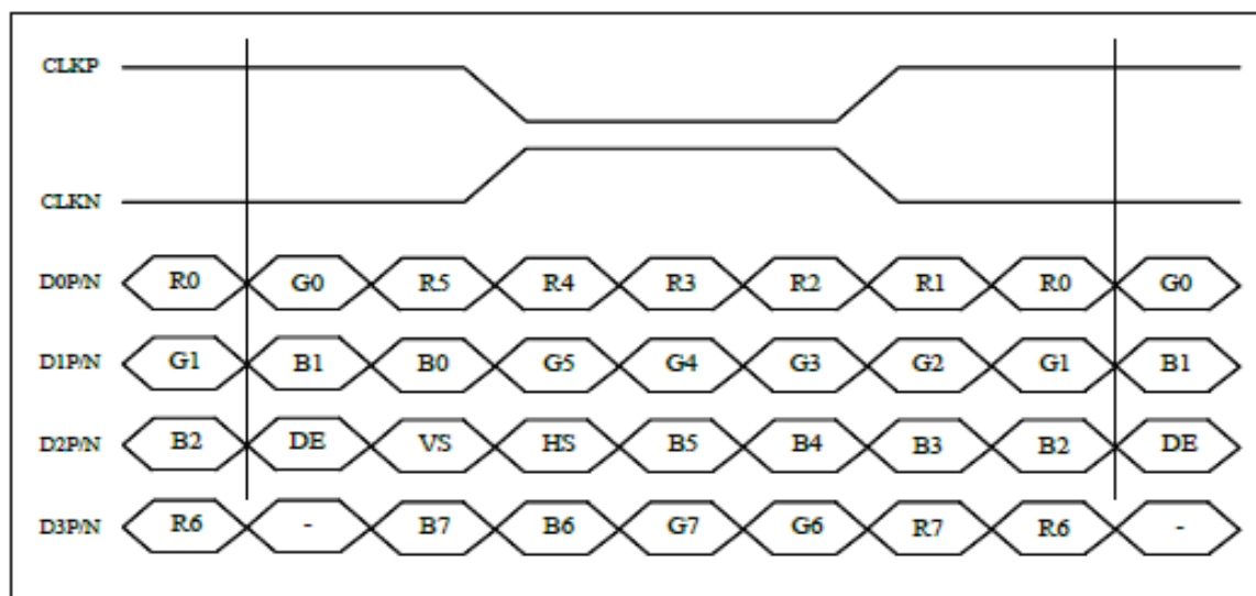
Figure 11 Data Mapping
