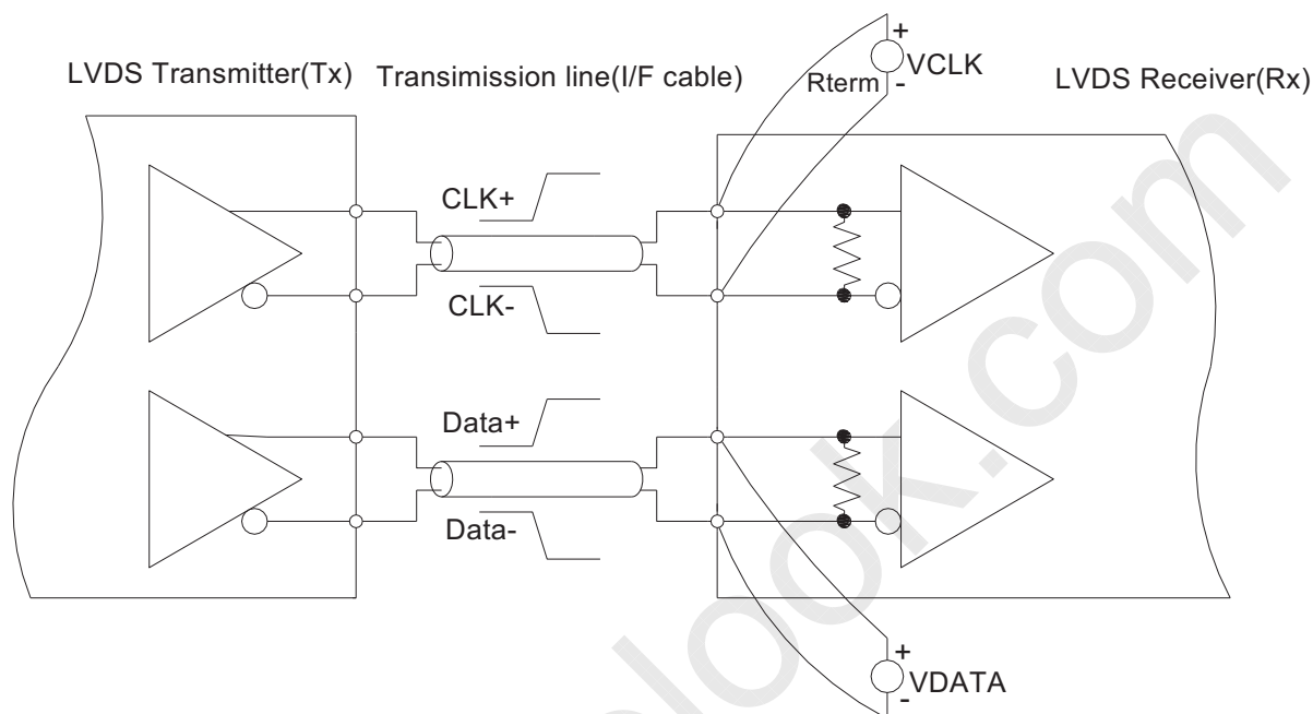
Figure 9 Measurement System
