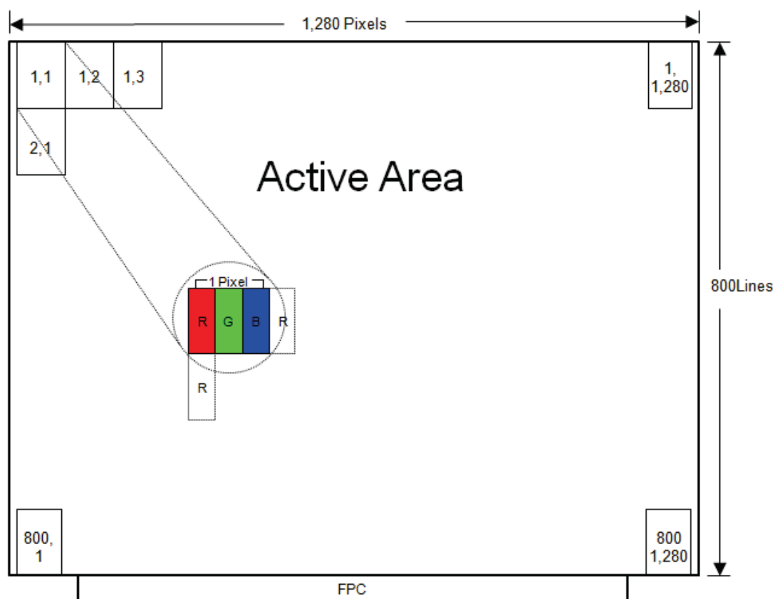
Figure2 Pixel Mapping
