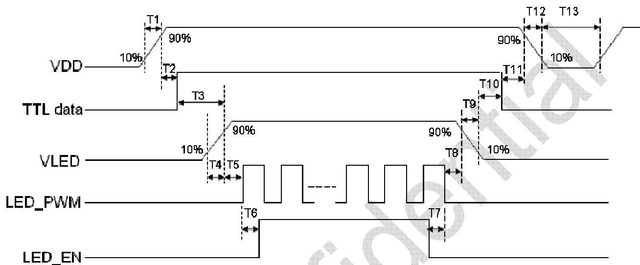
Figure 11 Power Sequence
