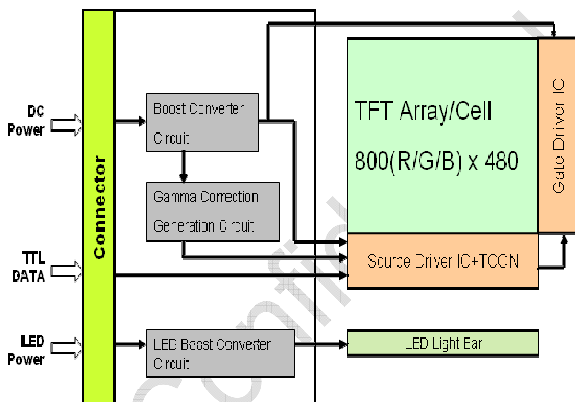
Figure 1 Block Diagram
