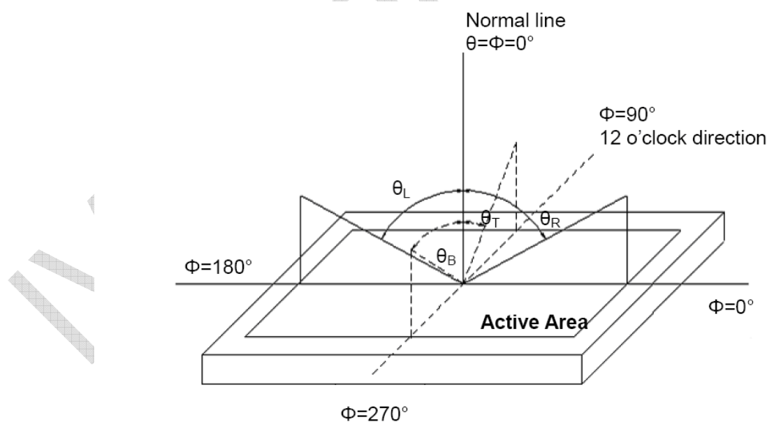
Figure 4 Definition of Viewing Angle
