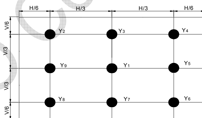
Figure 6 Measurement Locations
