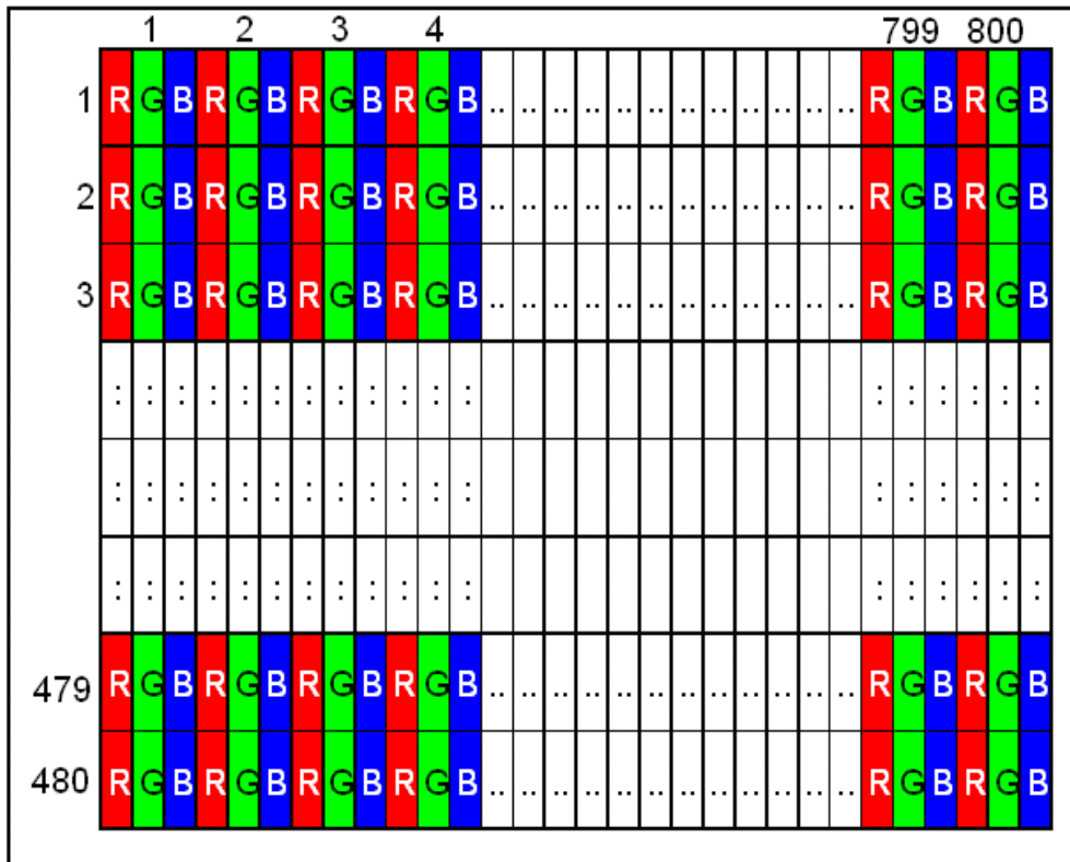
Figure 2 Pixel Format
