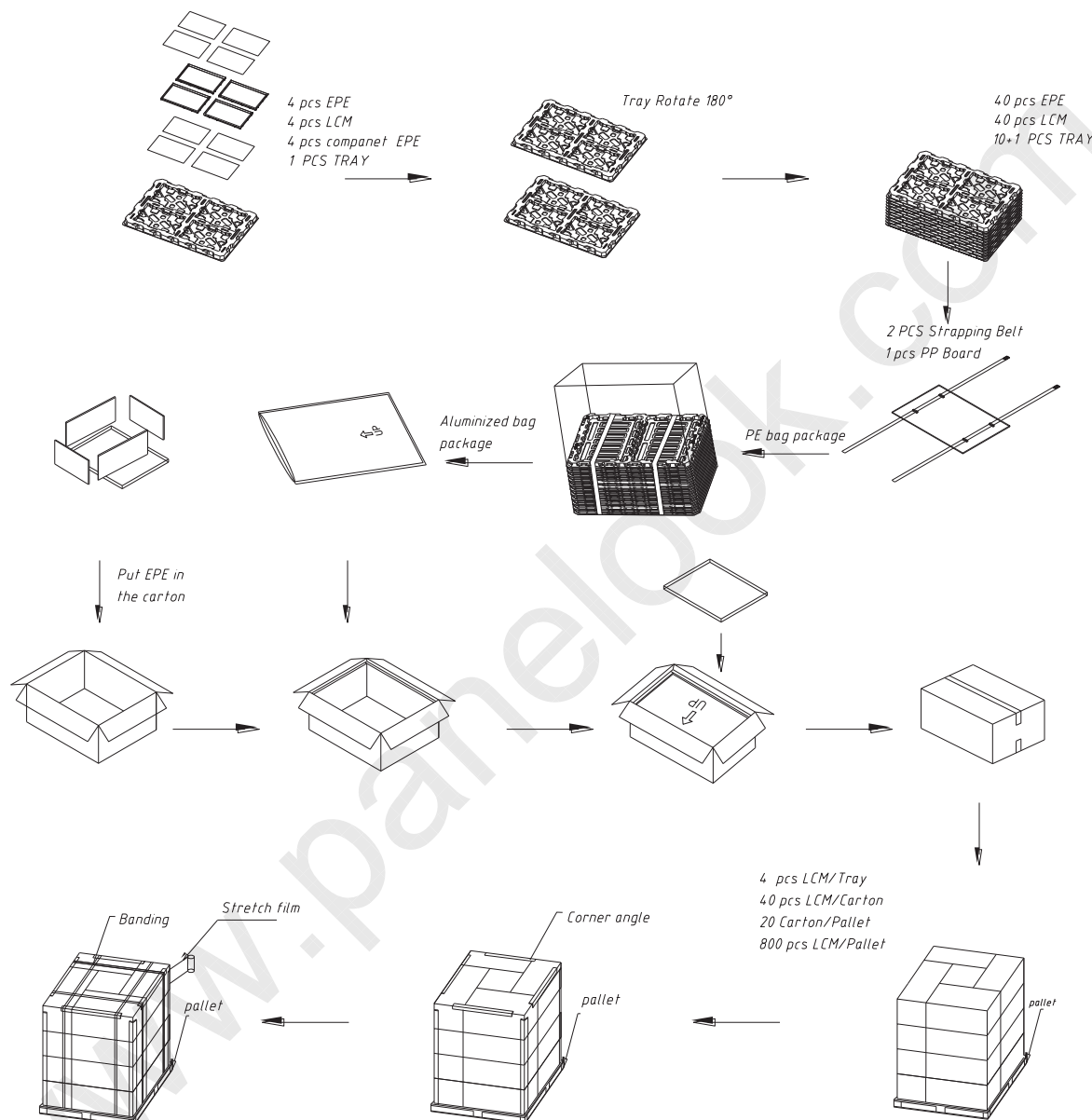
Figure 16 Packing Method
