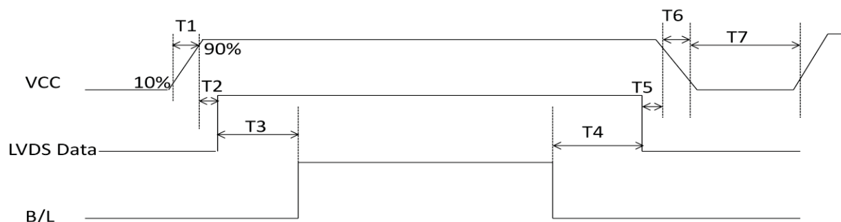
Figure 13 Power Sequence
