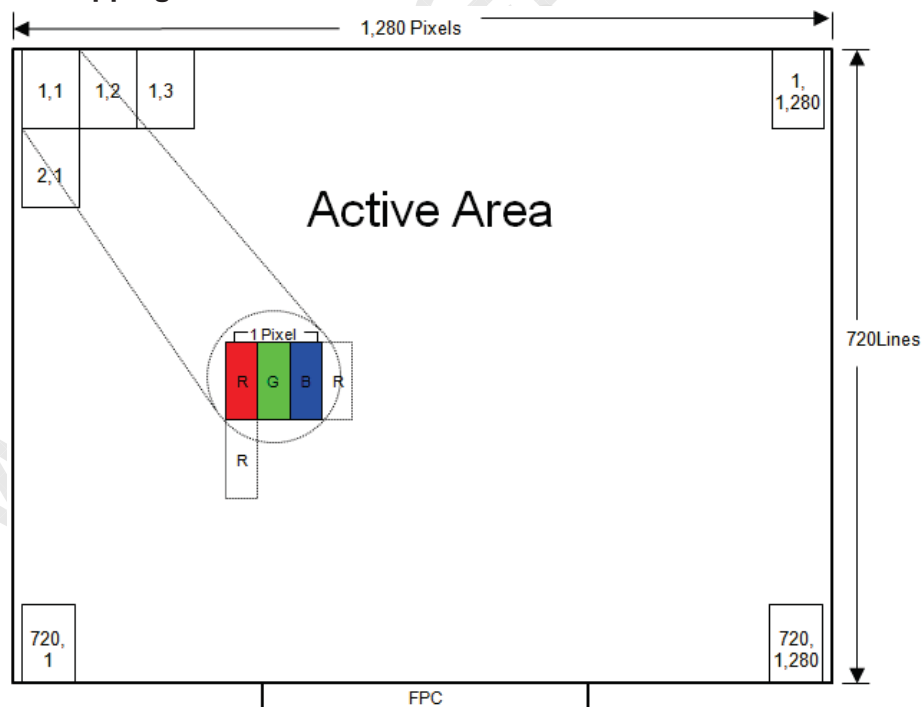
Figure 2 Pixel Mapping
