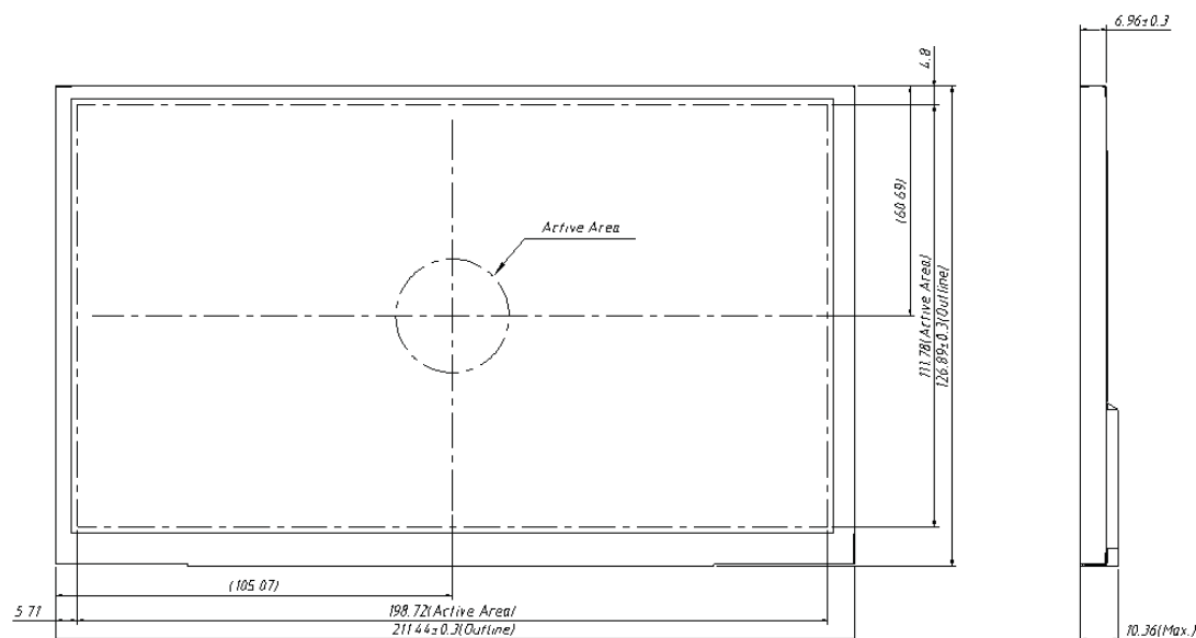
Figure 14 Reference Outline Drawing (Front Side)
