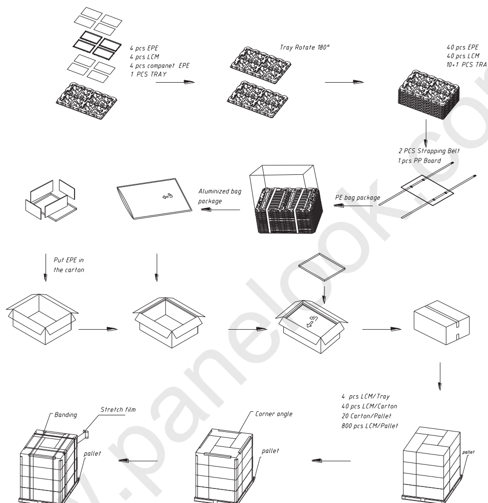
Figure 17 Packing Method
