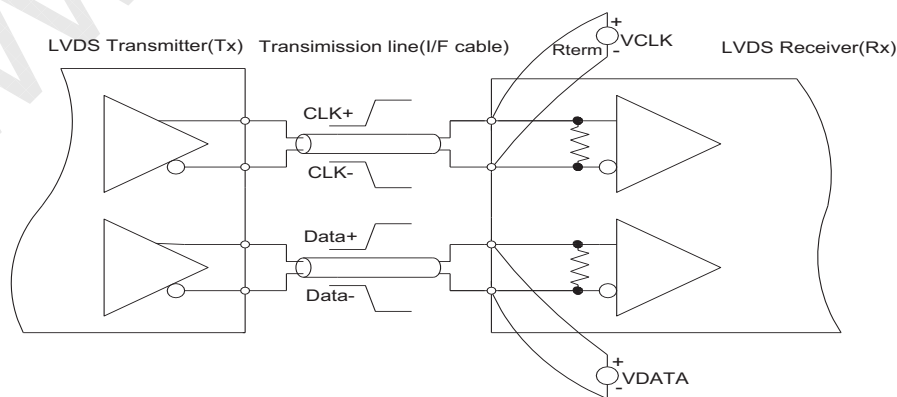
Figure 9 Measurement System
