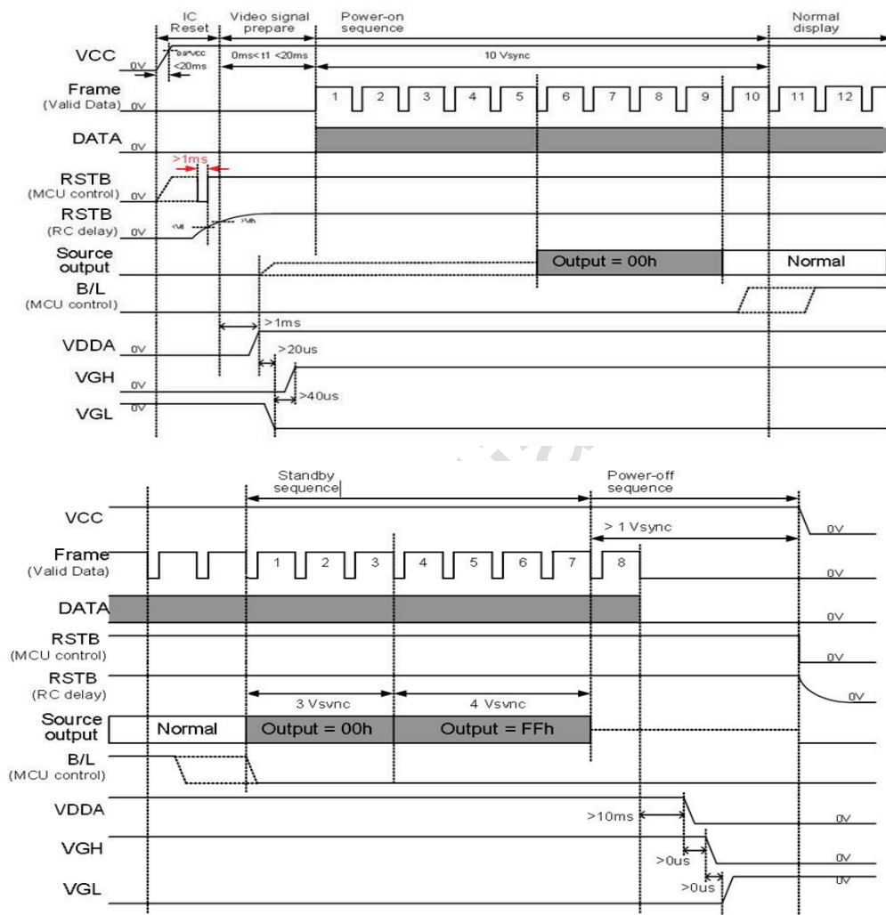
Figure 11 Power Sequence
