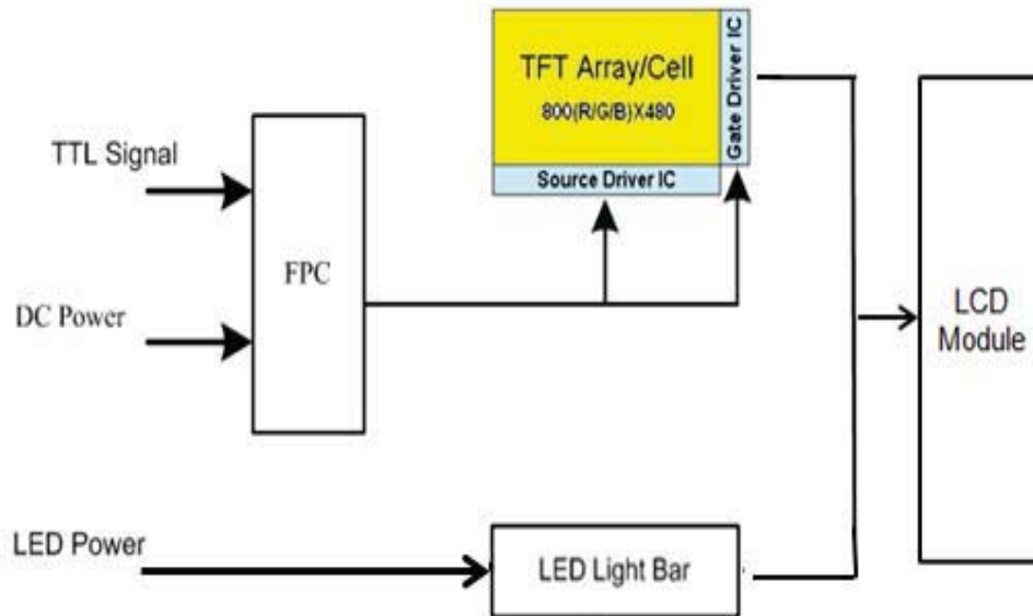
Figure 1 Block Diagram
