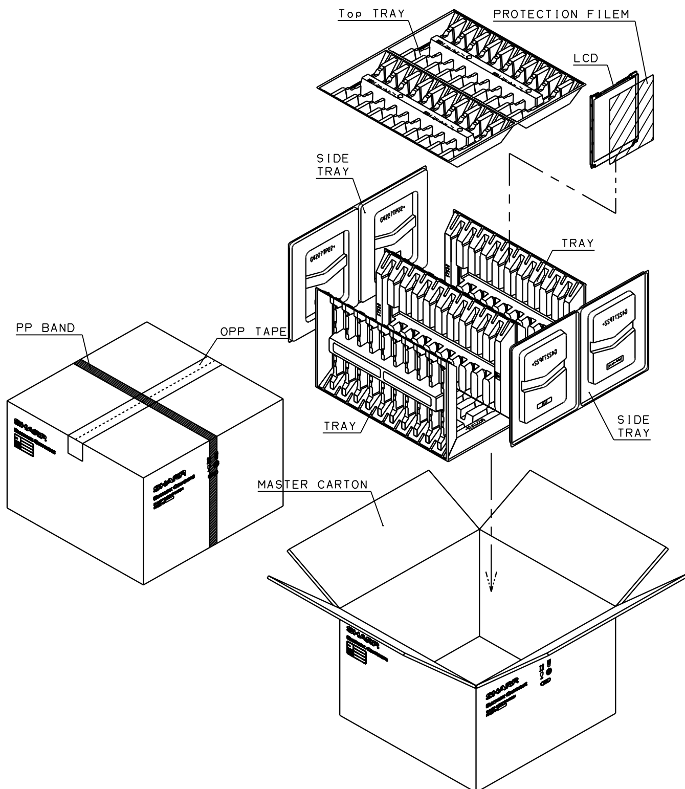
Fig.3 : PACKING FORM
