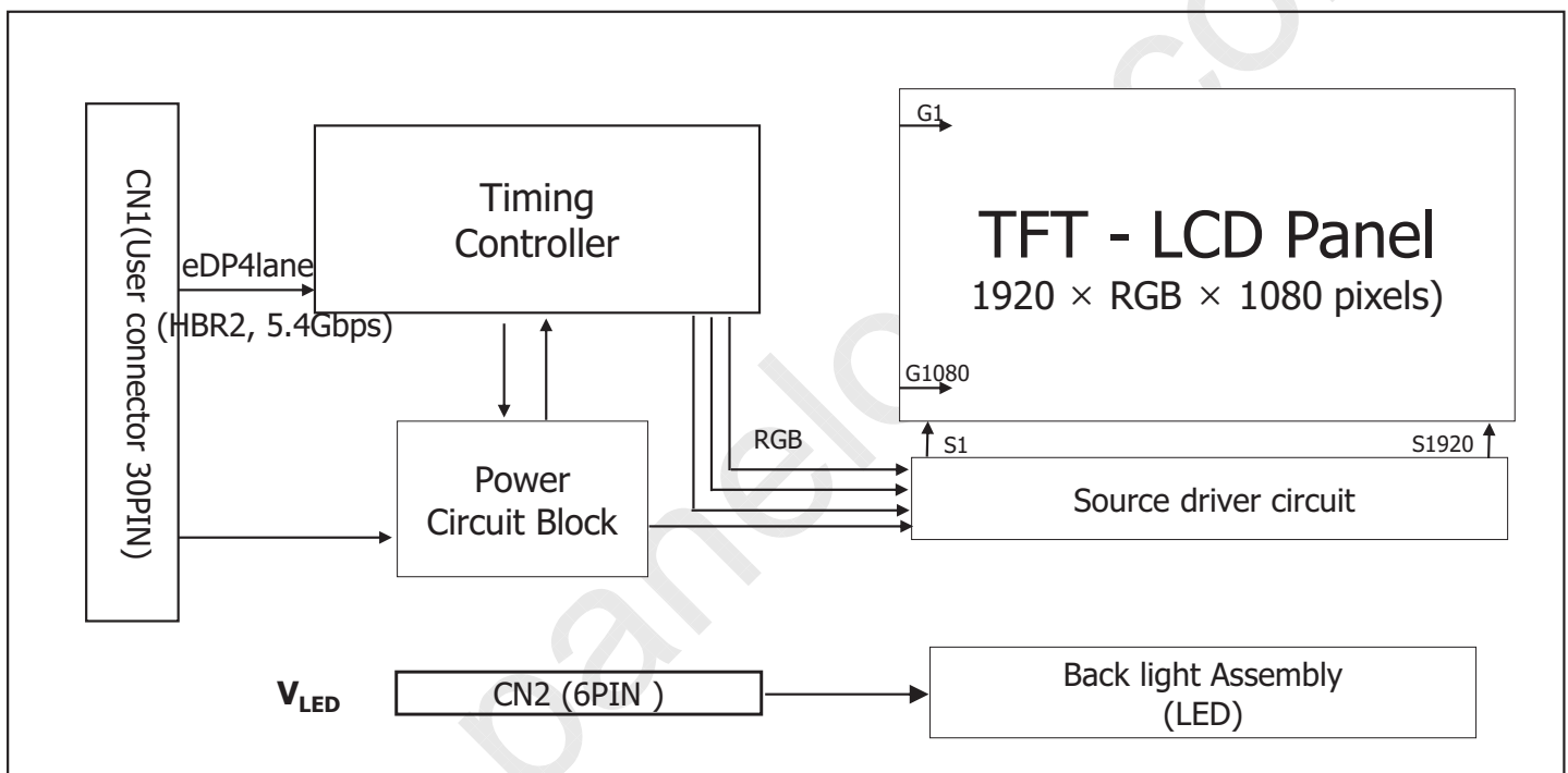
General Features [ FIG.1 ] Block diagram
