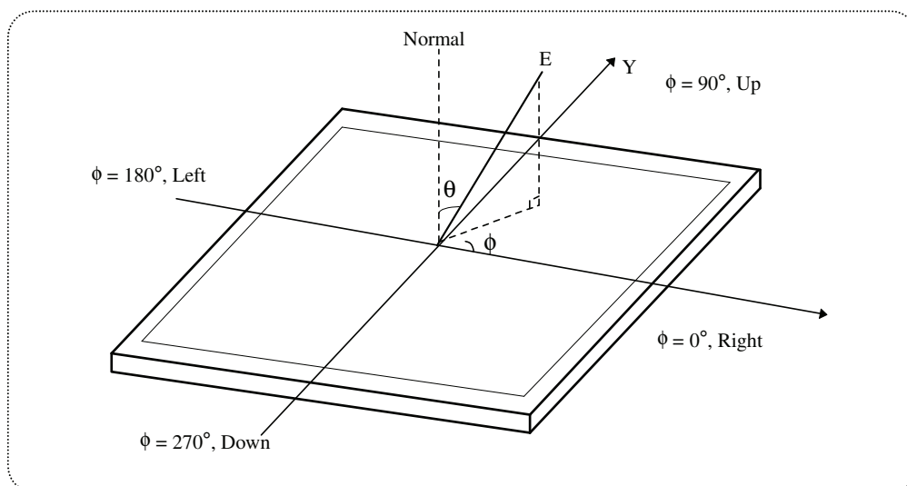
FIG.10 Viewing angle
