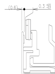
SECTION D-D SCALE 3/1
