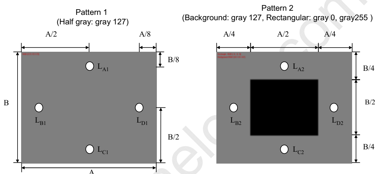
Figure 13. Crosstalk
