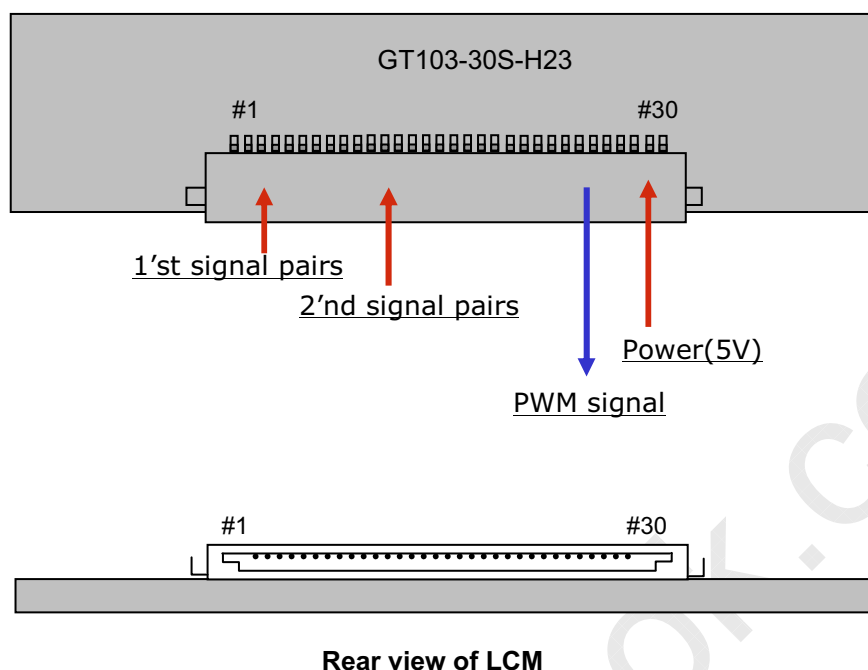
[ Figure 4 ] Connector diagram
