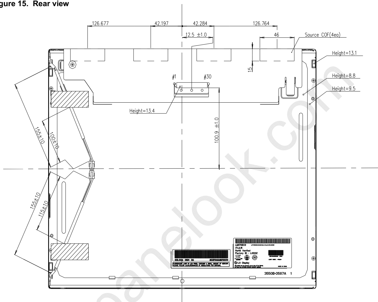
Figure 15. Rear view
