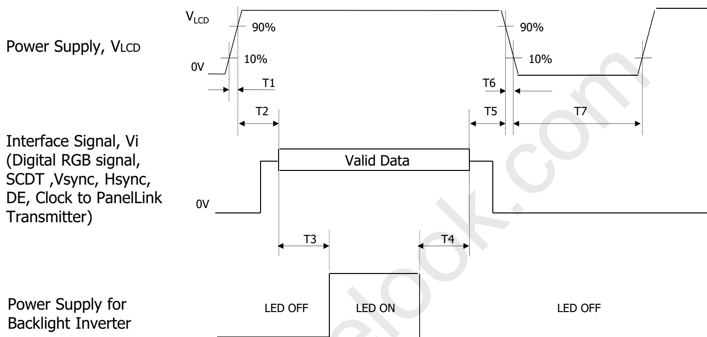
FIG.5 Power sequence
