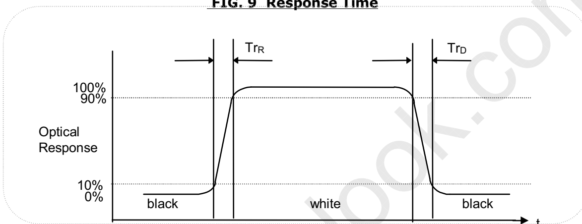
FIG. 9 Response Time
