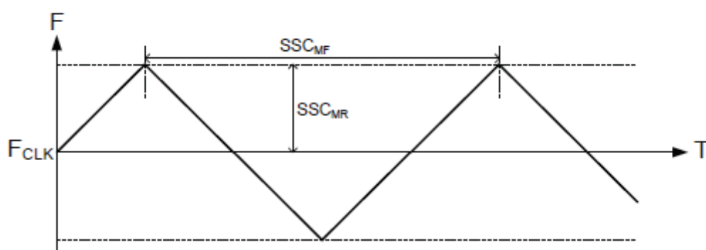
Figure 3-6. Frequency Modulation
