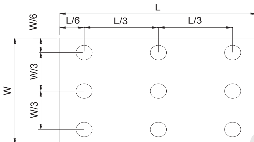
Fig. 4-4 Definition of measuring points
