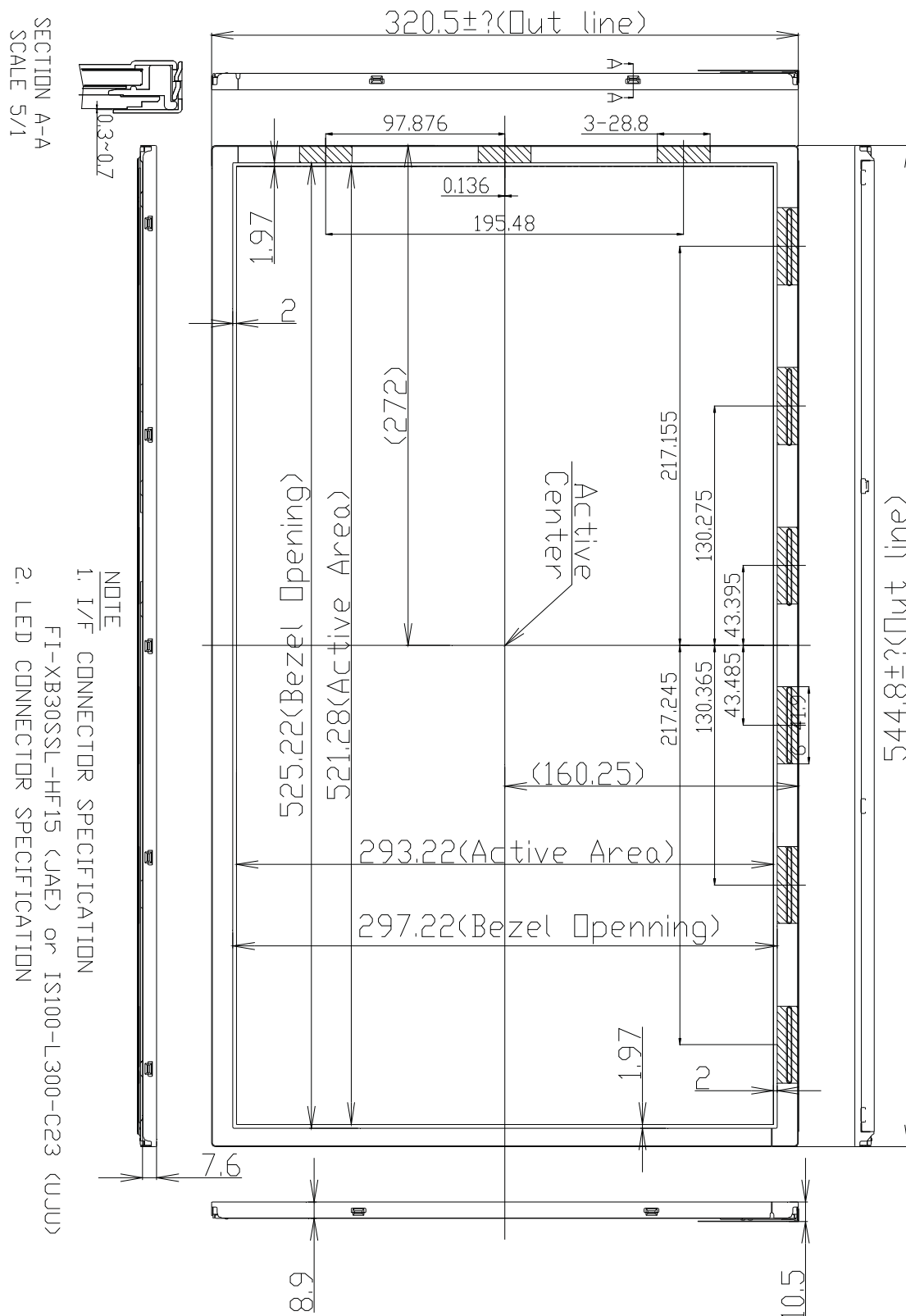
Figure 5. TFT-LCD Module Outline Dimensions (Front view)
