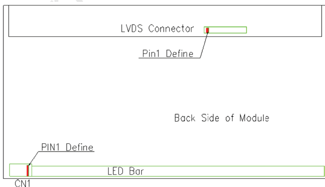
Figure2. Back Side of Module
