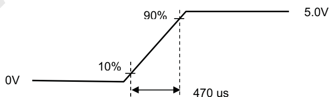
VCC rising time
