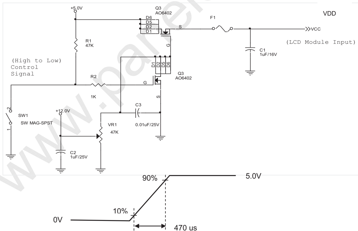
VDD rising time
