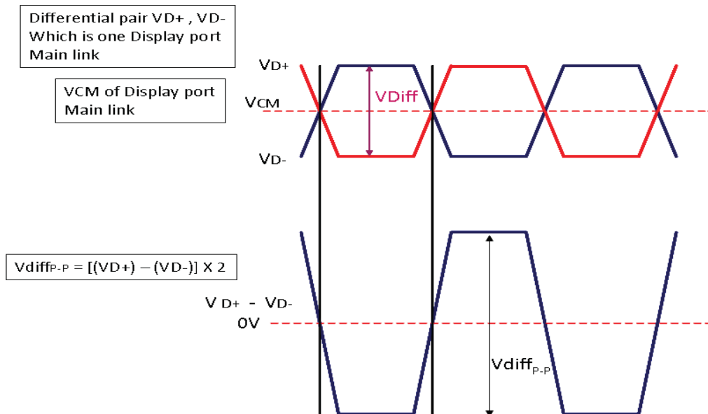
Display port main link
