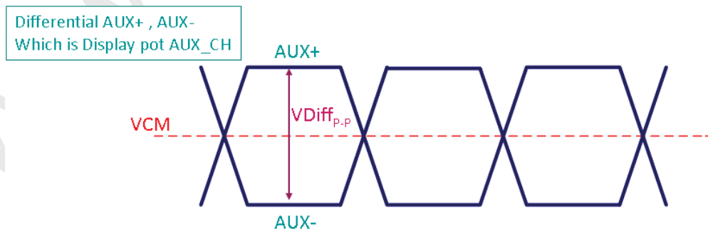
Display port AUX_CH
