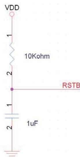
Fig. 6-3 Active Low
