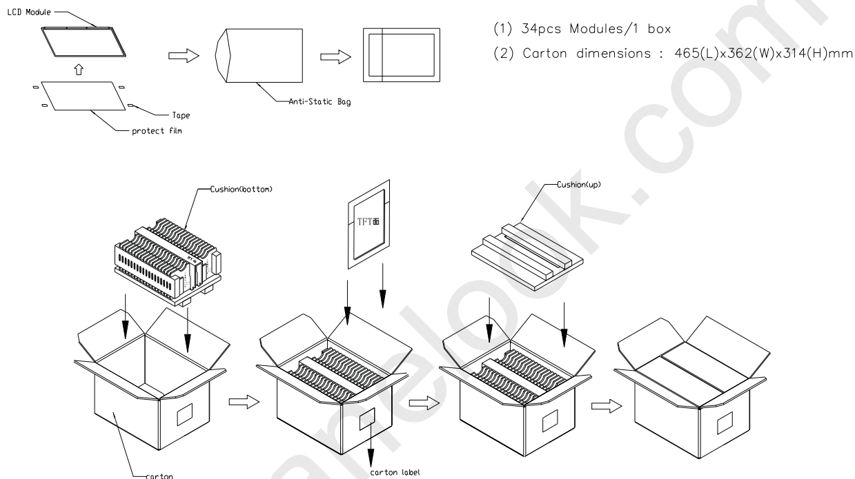
Figure. 9-1 Packing method
