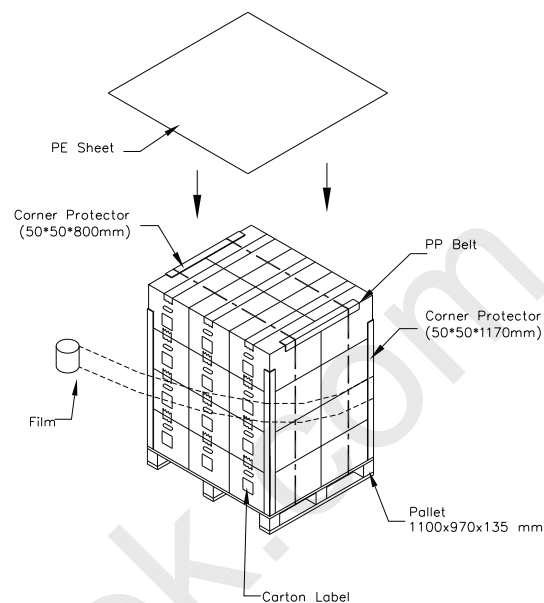
Figure. 9-2 Packing method
