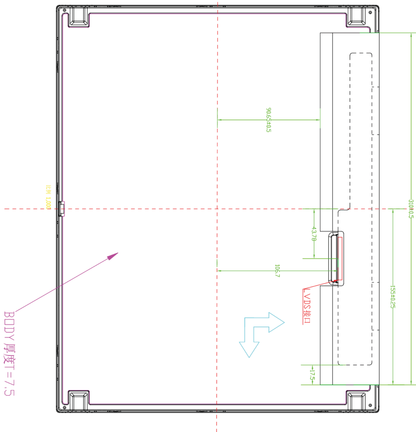
< Figure 4.TFT-LCD Module Outline Dimensions (Rear View) >
