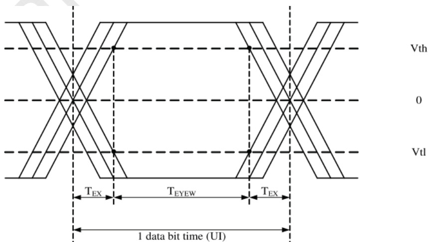
LVDS input eye diagram
